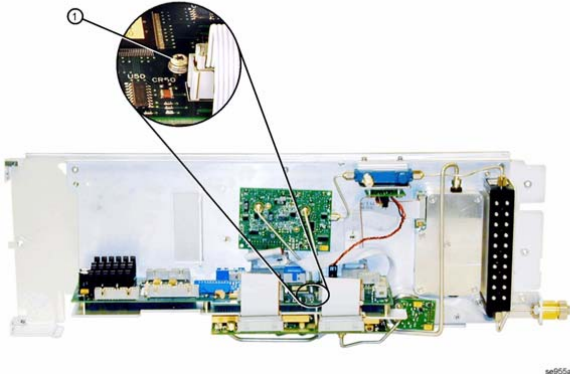
Figure 3-25 E8247D/57D Microcircuit Interface Deck Top View
