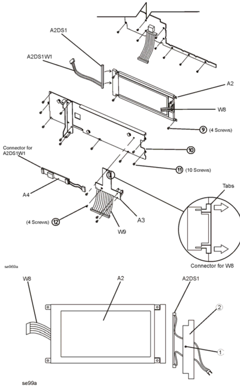
Figure 2-6 A2DS1 Display Backlight Removal
